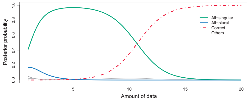
Fig. 5. Learning results for a singular/plural system.
