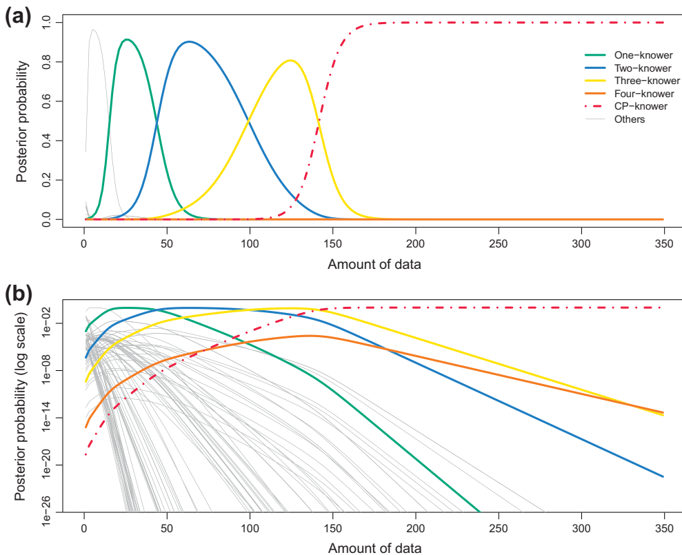
Fig. 3. (a) shows marginal posteriors probability of exhibiting each type of behavior, as a function of amount of data and (b) shows the same plot on a log y-axis demonstrating the large number of other numerical systems which are considered, but found to be unlikely given the data.
