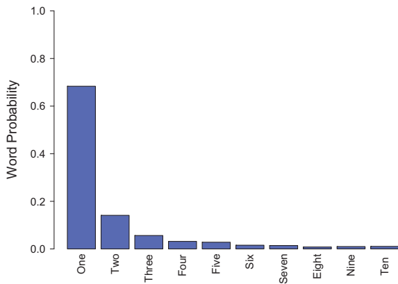
Fig. 2. Number word frequencies from CHILDES (MacWhinney, 2000) used to simulate learning data for the model.
