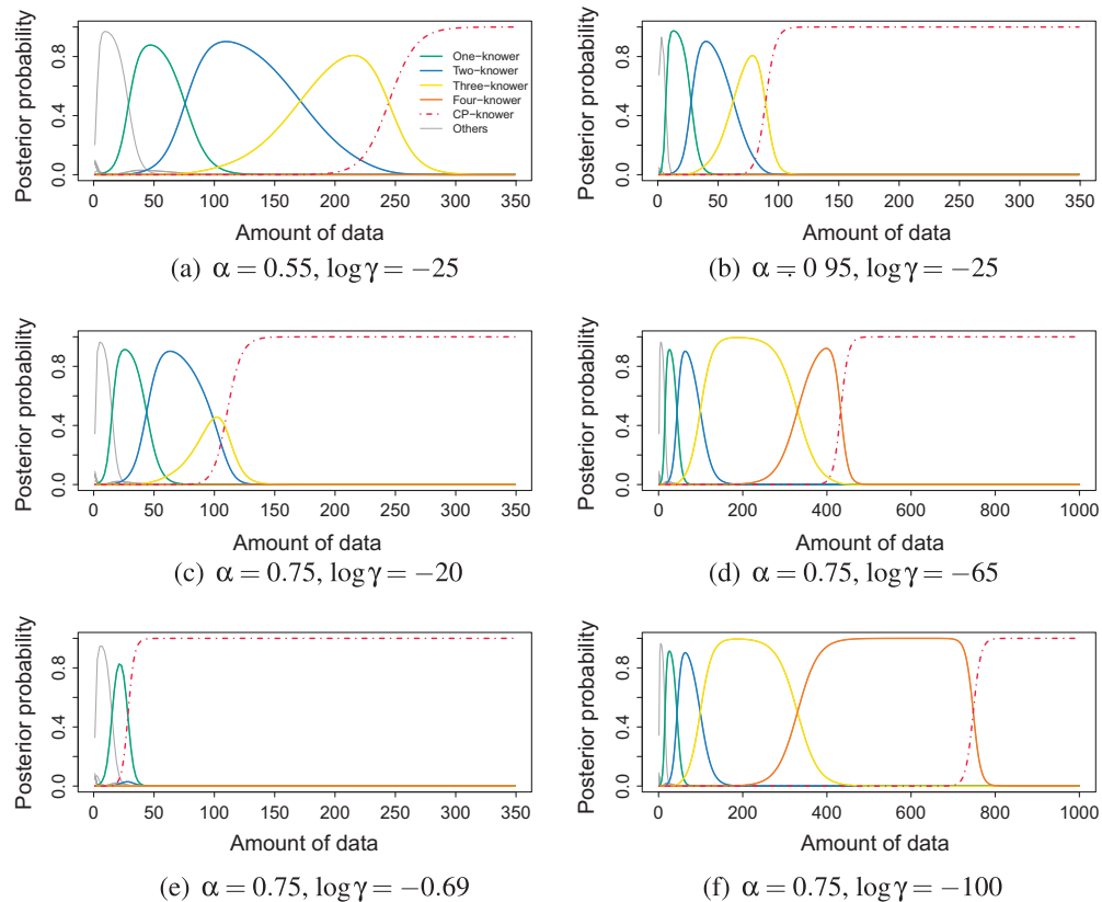
Fig. 4. Behavioral patterns for different values of \alpha and \gamma . Note that the x-axis scale is different for d and f.
