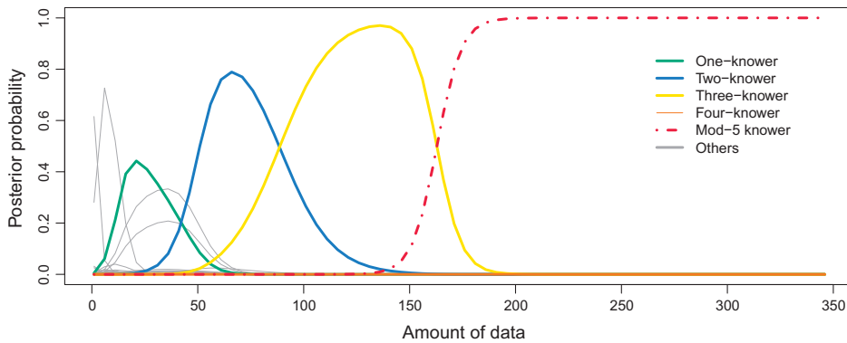
Fig. 6. Learning results for a Mod-5 system.
